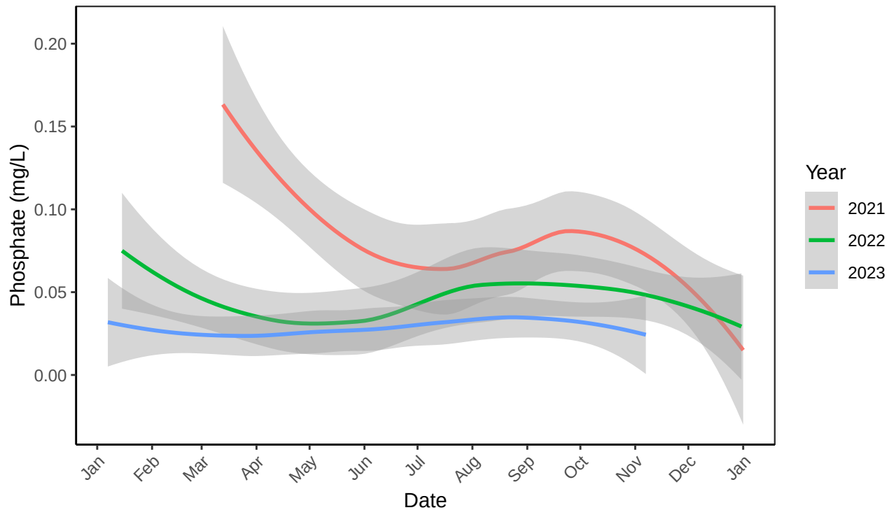
B2 Raceway 2 Phosphate (mg/L)
